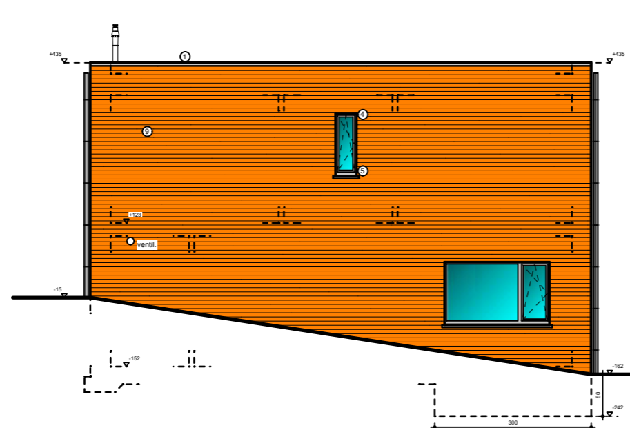
FACADE LATERALE
