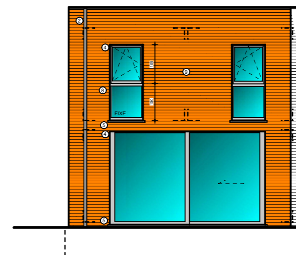
FACADE ARRIERE
